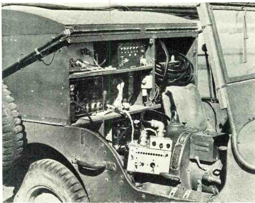
Closeup of jeep control station showing the control box in the foreground.
