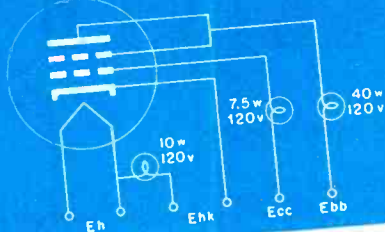
AGING SCHEDULE FOR HYTRON 50L6GT
