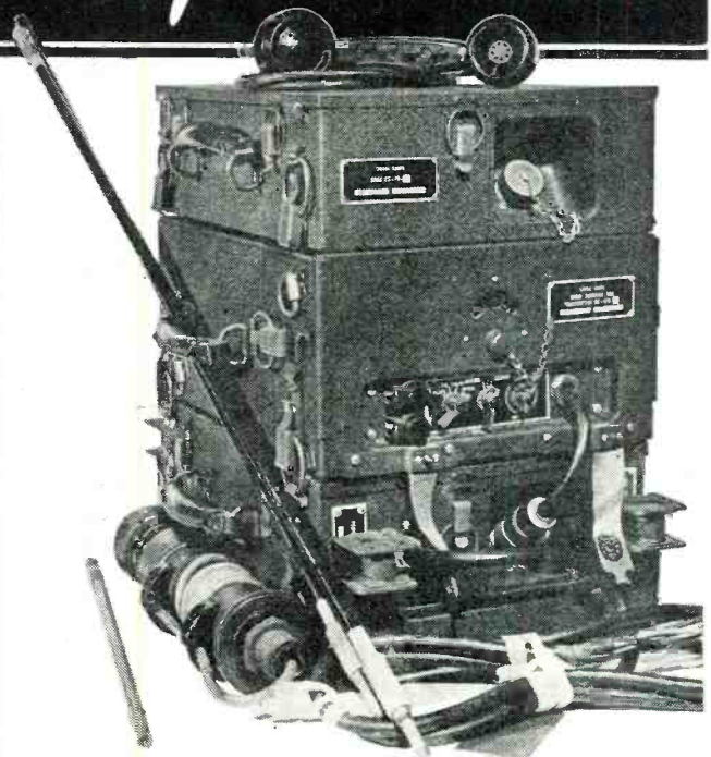
RADIO SET SCR-510 Brand-New
